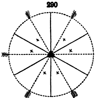
Symmetry of Rhombohedral-Hemimorphic Class
